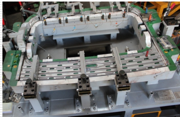
Automotive use wooden gauge
